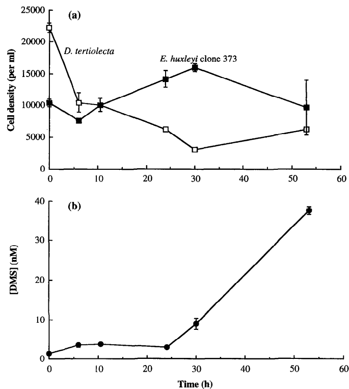
Fig. 7. Experiment with Oxyrrhis marina grazing both Dunaliella tertiolecta and Emiliania huxleyi clone 373. [a.] Prey cell densities. [b.] DMS concentrations. Numbers are means of duplicates, with ranges shown by error bars.
