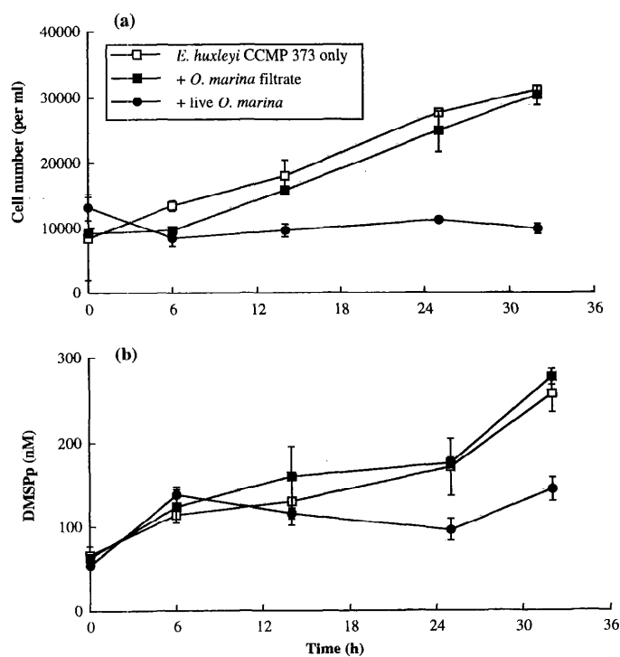
Fig. 6. Removal of prey cells (a) and prey DMSP (b) during grazing Oxyrrhis marina on Emiliania huxleyi clone 373. Numbers are means of duplicates, with ranges shown by error bars.
