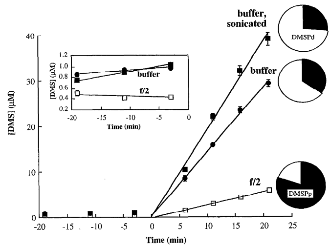
Fig. 4. Comparison of production of DMS from DMSP by Emiliania huxleyi clone 373 during resuspension into f/2 or MES buffer, with and without sonication; 1 mM DMSP was added at 0 min. Inset shows production of DMS from endogenous DMSP by cells resuspended in MES buffer before addition of DMSP. Pie graphs show relative fractions of particulate DMSP (■, DMSP p ) and dissolved DMSP (□, DMSP d ) found following resuspension in each case. Numbers are means of duplicates, with ranges shown by error bars.
