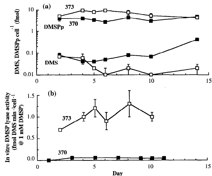
Fig. 3. Comparison of Emiliana huxleyi clones 370 (■) and 373 (□) during batch growth. [a.] Particulate DMSP and DMS per cell vs. time. [b.] In vitro DMSP lyase activity per cell vs. time. Numbers are means of duplicates, with ranges shown by error bars.
