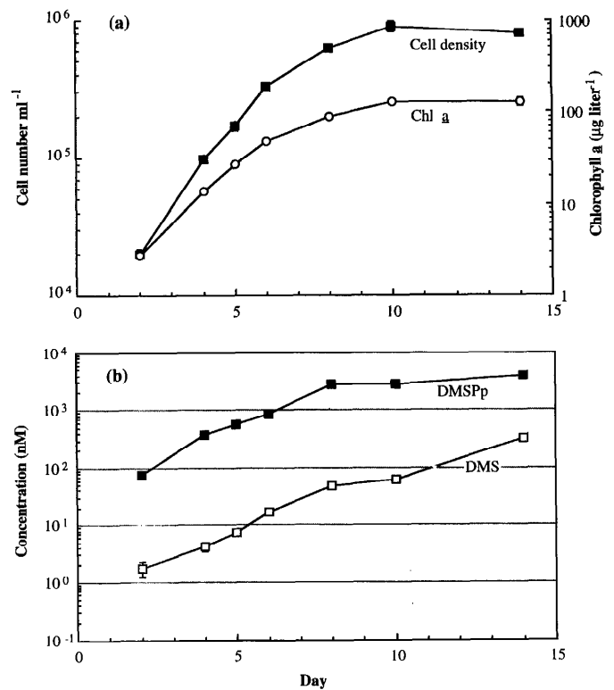
Fig. 1. Emiliana huxleyi clone 370 during batch growth. [a.] Cell density and chlorophyll a vs. time. [b.] DMS and particulate DMSP vs. time. Numbers are means of duplicates, with ranges shown by error bars.
