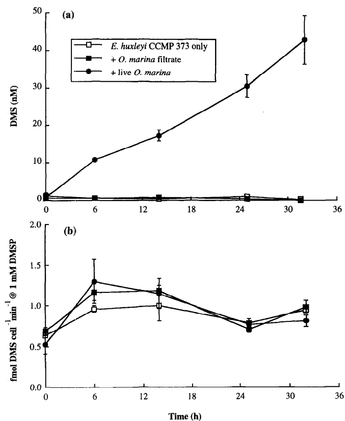
Fig. 5. Production of DMS (a) and in vitro DMSP lyase activity per cell (b) during grazing of Oxyrrhis marina on Emiliania huxleyi clone 373. Numbers are means of duplicates, with ranges shown by error bars.
